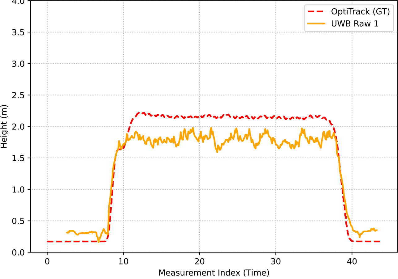
Z-Axis (Altitude) Stability Profile
